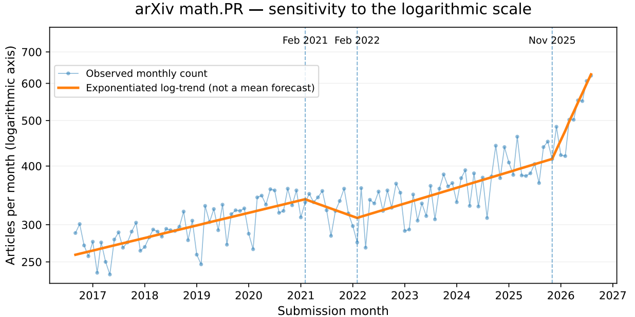
Figure 3: Global variant fitted to logarithms and displayed on a logarithmic axis. The exponentiated trend is geometric. The recent acceleration is recovered, but the earlier breakpoints and the final date differ from those in the count model.
