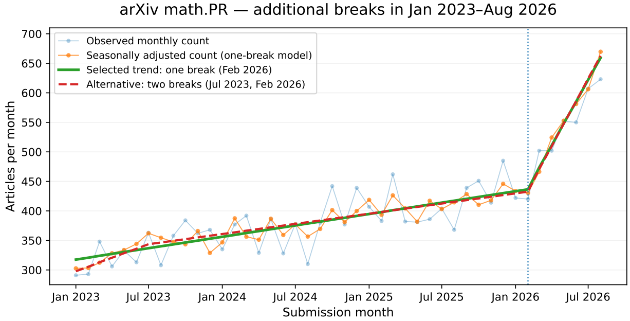
Figure 6: Comparison of the local one-break and two-break models. The seasonally adjusted counts use the monthly effects of the one-break model. The two-break model has its own seasonality, re-estimated jointly: the two adjustments are not assumed to be identical.
