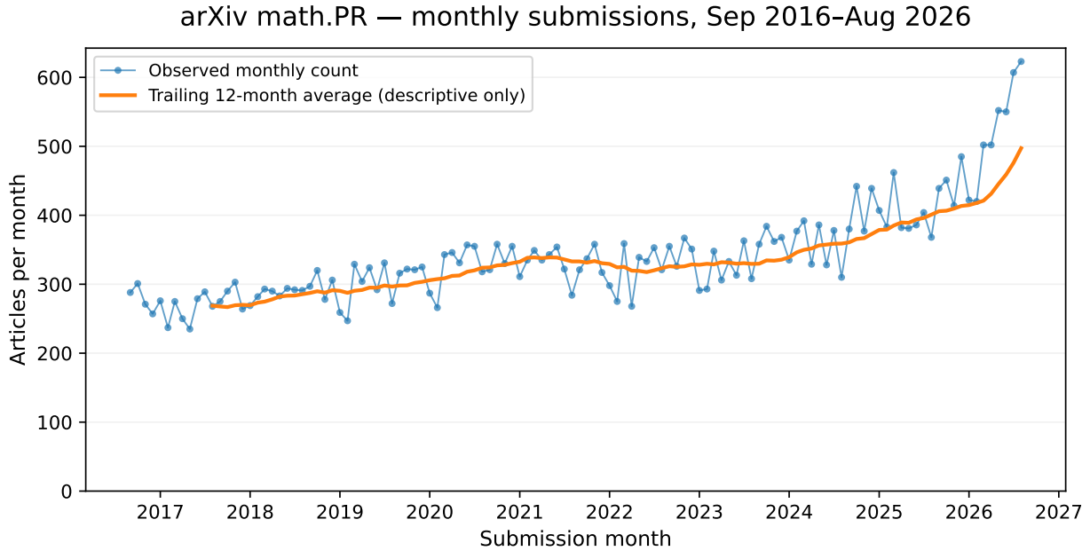
Figure 1: Observed monthly counts and trailing twelve-month moving average. The vertical axis starts at zero. September–December 2026 are neither observed nor extrapolated. Source: arXiv metadata; monthly observations in Appendix A.
