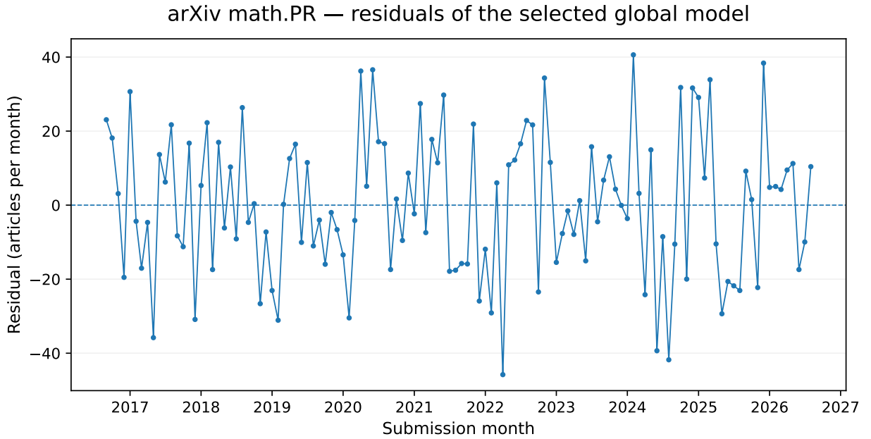
Figure 5: Residuals from the selected global fit. The zero line is not a confidence bound; no calibrated test band is shown.
