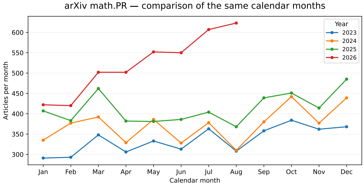
Figure 7: Comparison of the same months over 2023–2026. Autumn increases recur before 2026. The 2026 series ends in August; no autumn continuation is assumed.
