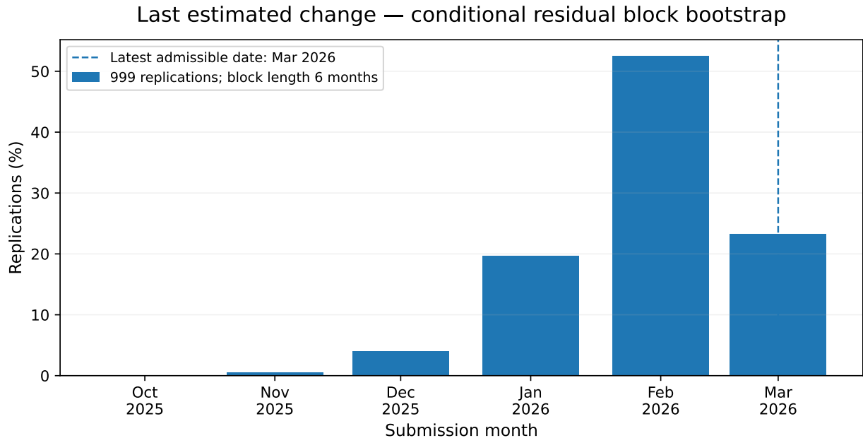
Figure 4: Conditional bootstrap distribution of the final date. The mass at the right-hand boundary, March 2026, also reflects the final-segment length constraint.
