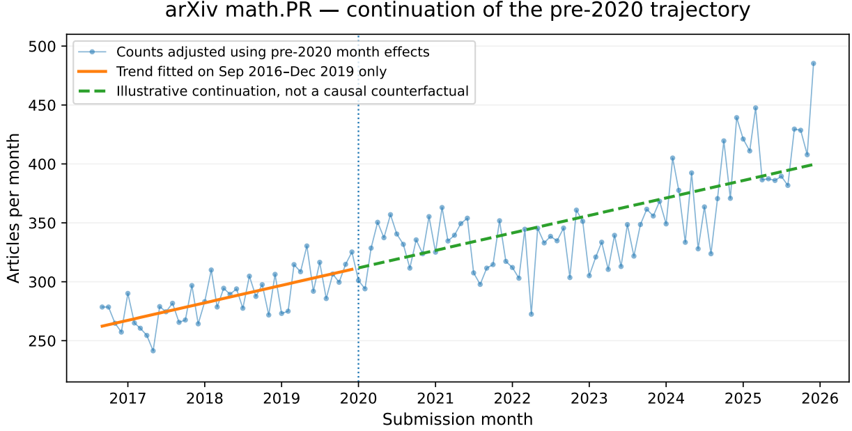
Figure 8: Trajectory fitted before 2020 and illustrative extension through 2025. Observed counts are adjusted using only monthly effects estimated before 2020. The vertical line marks the start of the period not used for estimation. No prediction interval or causal effect is shown.
