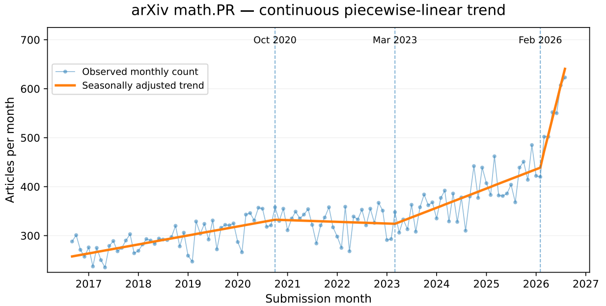
Figure 2: Main global model: observed counts and continuous seasonally adjusted trend. The estimated breakpoints are October 2020, March 2023 and February 2026. The vertical axis is restricted to make slope changes visible; Figure 1 provides a view starting at zero.
